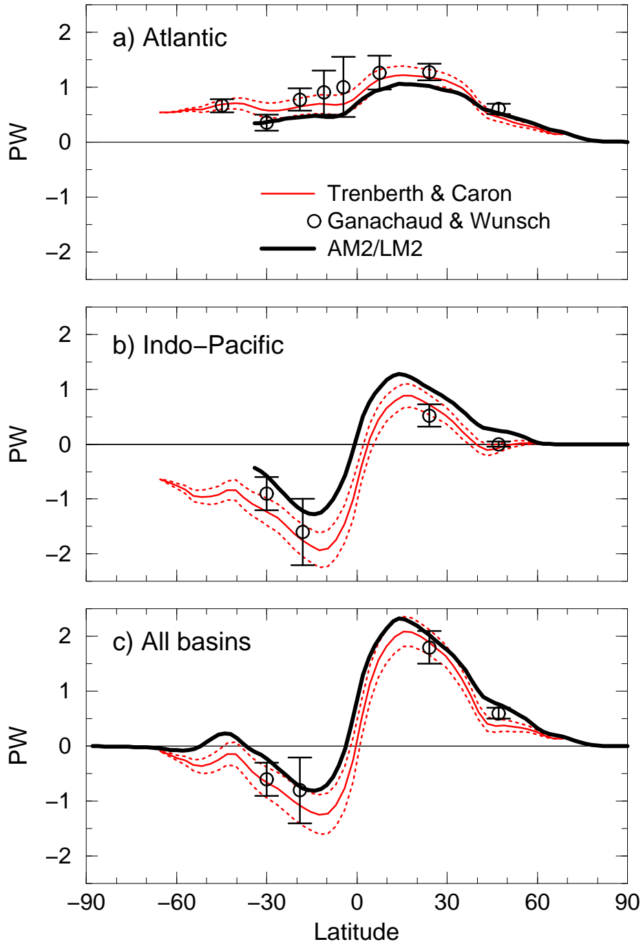
Figure 22. Poleward oceanic heat transport in petawatts ( 10^{15} W) from observational based estimates and implied by AM2/LM2 (dark black line). The observed estimates are derived from atmospheric data (Trenberth and Caron 2001; red lines with dashed lines indicating plus or minus one standard error; based on NCEP-derived products) or oceanic data (Ganachaud and Wunsch 2003). Results are shown for the a) Atlantic, b) Indo-Pacific, and c) world ocean basins.
