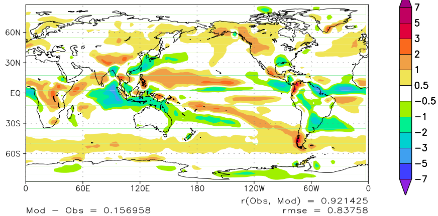
Figure 8. Annual long-term mean precipitation in \text{mm d}^{-1} for (a) AM2/LM2, (b) CMAP observations, and (c) AM2/LM2 minus CMAP. Statistics at the bottom of (a) and (b) include the global mean and standard deviation. Statistics at the bottom of (c) include the difference in global means, the correlation coefficient, and the root mean square error.
