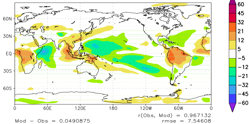
Figure 9. Annual long-term mean outgoing longwave radiation (OLR) in W m -2 for (a) AM2/LM2, (b) ERBE observations, and (c) AM2/LM2 minus ERBE. Statistics at the bottom of (a) and (b) include the global mean and standard deviation. Statistics at the bottom of (c) include the difference in global means, the correlation coefficient, and the root mean square error.
