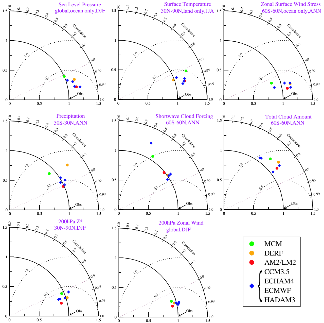
Figure 21. Taylor diagrams for selected variables comparing the skill of AM2/LM2 (red circle) in reproducing the observed climatology to that of older GFDL models (MCM and DERF, green and orange circles respectively) and other models participating in AMIP II (CCM3.5, ECHAM4, ECMWF, and HADAM3). Note that all non-GFDL models are plotted with a blue diamond to prevent unique identification. The selected variables include those associated with surface climate (SLP, land surface air temperature, and oceanic wind stress, top row), water cycle and clouds (precipitation, shortwave cloud forcing, and total cloud amount, middle row), and upper tropospheric circulation (200 hPa eddy geopotential and zonal wind, bottom row). The observational sources for these data include the NCEP reanalyses for SLP and 200 hPa eddy geopotential and zonal wind, ECMWF reanalyses for oceanic wind stress, ERBE for cloud radiative forcing, ISCCP for total cloud amount, CMAP for precipitation and CRU for land surface air temperature. Beneath each variable name is an indication of the geographical domain and season used in the calculation.
