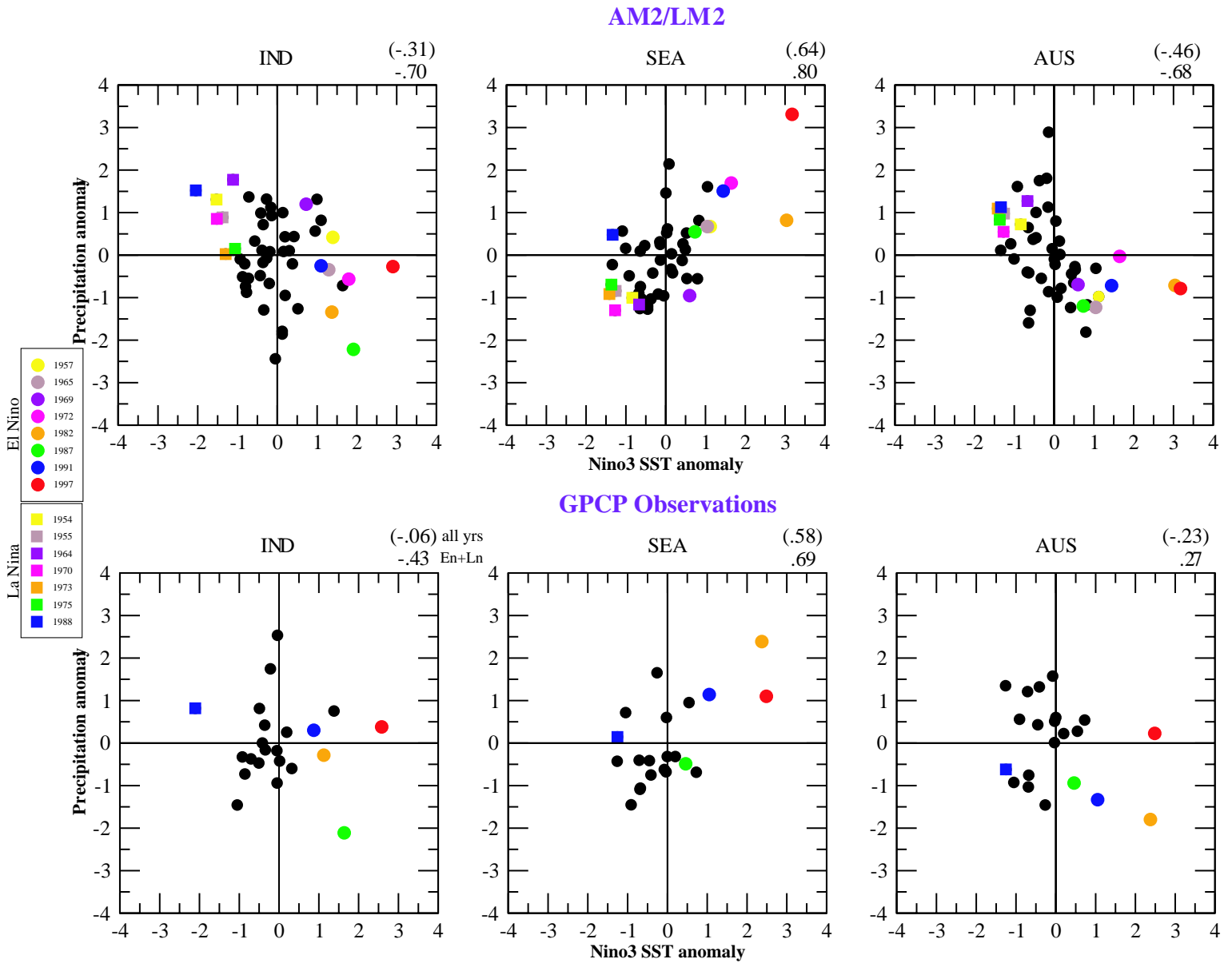
Figure 16. Scatterplots of the precipitation anomalies in three monsoon regions [IND - Indian; AUS - northern Australia; SEA - southeast Asia; boundaries of these regions are depicted in Figure 3 of Lau and Nath (2000)] versus the NINO3 SST anomalies. The abscissa in all panels represents the standardized SST anomaly in the NINO3 region. The ordinate axis represents the standardized precipitation anomaly in IND during the JJA season (left panels), and in SEA (middle panels) and AUS (right panels) during the DJF season. The upper panels are based on AM2/LM2 output for the 1951-2000 period. The lower panels show the observational estimates provided by GPCP for the shorter period of 1979-2000. In each panel, the anomalies of precipitation and NINO3 index for a given year are jointly depicted by a small dot or square. The outstanding warm and cold ENSO events are highlighted using colored dots and squares, respectively. The data for all remaining years are plotted using black dots. The correlation coefficient for the data entries in each panel is shown in the upper right corner of that panel. Correlation values based on all available years are given in parentheses. Correlation values based on the available warm and cold ENSO events only are given without parentheses.
