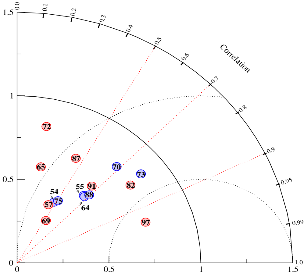
Figure 15. Taylor diagram depicting the relationships between the observed DJF 200 hPa height anomalies in the North Pacific / North American sector ( 20^{\circ} - 70^{\circ} N, 60^{\circ} - 180^{\circ} W) during selected ENSO events and the corresponding ensemble-mean patterns as simulated in the 10-member AMIP-style runs with the AM2/LM2. Results for individual warm and cold ENSO events are presented using red and blue dots, respectively. The two-digit label for each dot indicates the year of the event in question. The spatial correlation coefficient is given by the cosine of the angle between the abscissa and the straight line joining the origin and the dot representing the event of interest; correlation values are given along the outer solid arc. The ratio between the simulated and observed spatial variances is given by the distance between the dot and origin; inner and outer solid arcs indicate ratios of 1 and 1.5, respectively. The root mean square (rms) difference between the simulated and observed pattern, as normalized by the spatial variance of the observed field, is given by the distance between the dot and the point with coordinates (1,0) in the diagram; inner and outer dotted arcs indicate normalized rms differences of 0.5 and 1, respectively.
