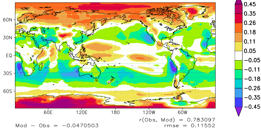
Figure 11. Annual long-term mean total cloud amount (fraction) for (a) AM2/LM2, (b) ISCCP observations, and (c) AM2/LM2 minus ISCCP. Statistics at the bottom of (a) and (b) include the global mean and standard deviation. Statistics at the bottom of (c) include the difference in global means, the correlation coefficient, and the root mean square error. Note that these statistics have been computed only over the domain 60°S-60°N, as high latitude ISCCP data is unreliable.
