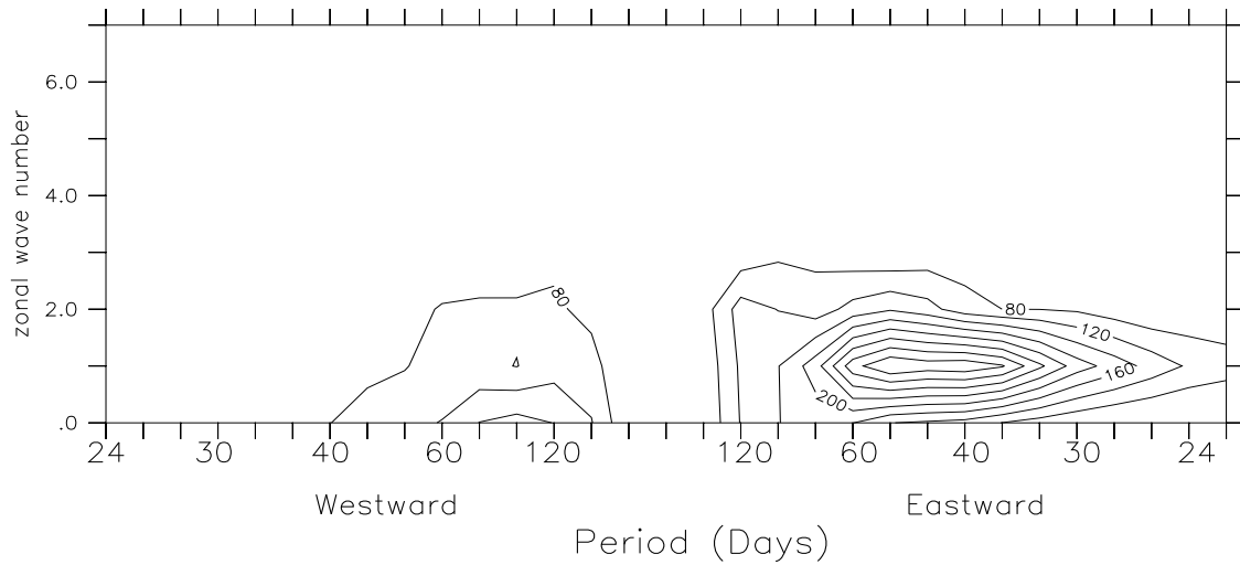
Figure 19. Wave frequency spectra of 5°N to 5°S 200 hPa zonal wind variance for AM2/LM2 (top) and NCEP reanalyses (bottom). Contour interval is 40 m 2 s -2 .
