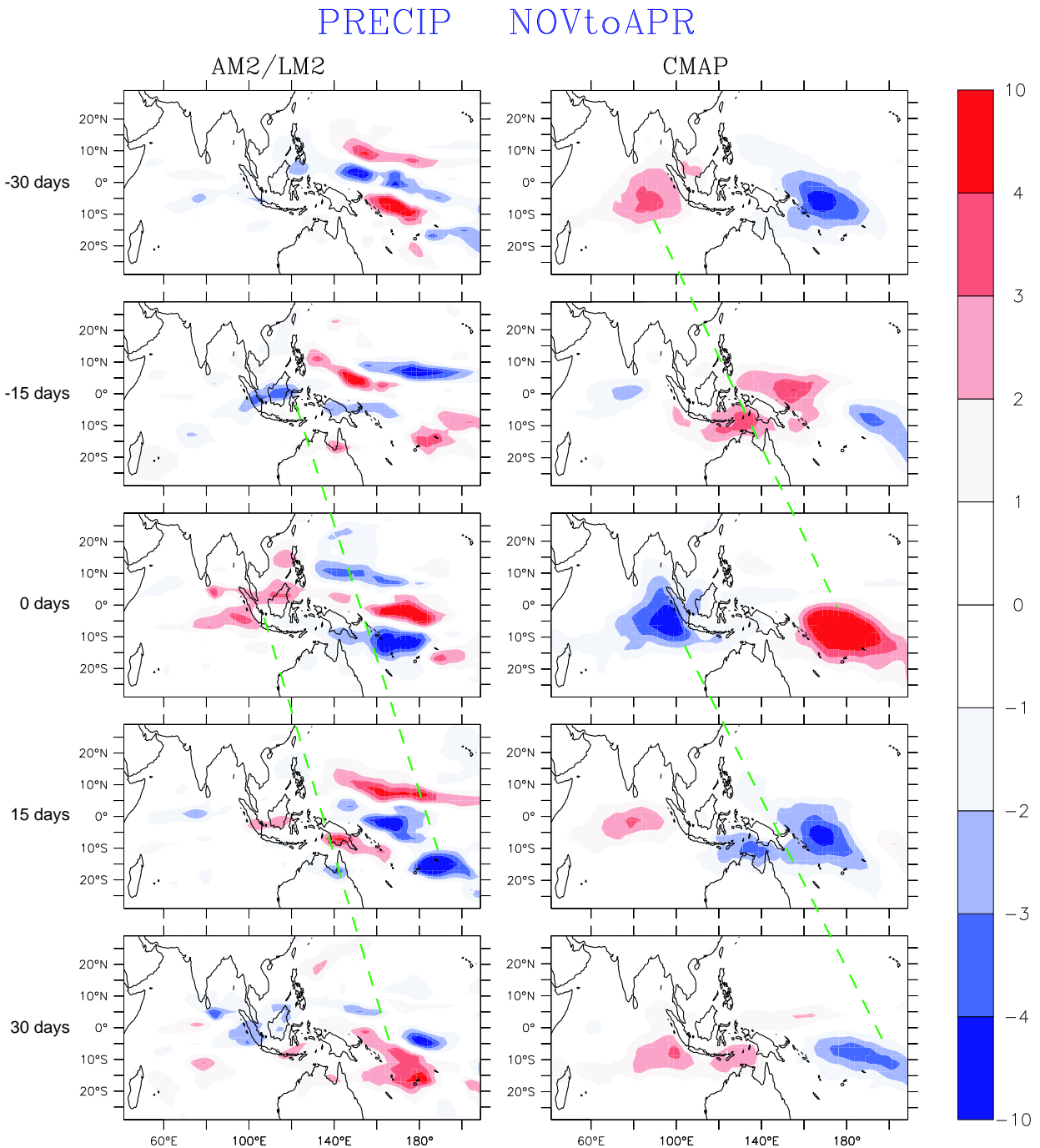
Figure 20. Composite Northern Hemisphere winter (November-April) Madden-Julian Oscillation from 30-90 day filtered precipitation in \text{mm d}^{-1} . Maps based on AM2/LM2 are shown in the left column and those based on CMAP observations in right column. Sequential maps are 10 day means centered on lags of -30 days, -15 days, 0 days, +15 days, and +30days. The superimposed green dashed lines indicate propagation of the disturbance. Note that the values for AM2/LM2 values have been enhanced by a factor of 2.
