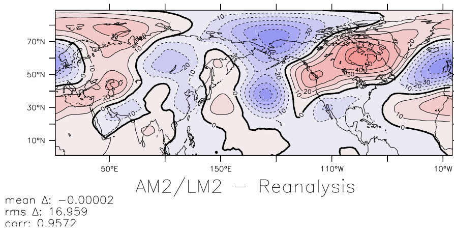
Figure 7. Long-term DJF mean departure of 500 hPa geopotential height from its zonal mean for (a) AM2/LM2, (b) NCEP/NCAR reanalysis climatology, and (c) AM2/LM2 minus NCEP. Contour interval is 25 m in (a) and (b) and 10 m in (c). Statistics at the bottom of (a) and (b) include the Northern Hemisphere mean and standard deviation. Statistics at the bottom of (c) include the difference in Northern Hemisphere means, the root mean square error, and the correlation coefficient.
