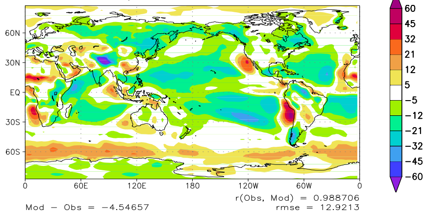
Figure 10. Annual long-term mean absorbed solar radiation (SWAbs) in W m -2 for (a) AM2/LM2, (b) ERBE observations, and (c) AM2/LM2 minus ERBE. Statistics at the bottom of (a) and (b) include the global mean and standard deviation. Statistics at the bottom of (c) include the difference in global means, the correlation coefficient, and the root mean square error.
