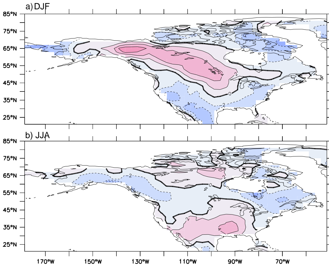
Figure 3. Long-term mean 2 m temperature difference for North America between CRU climatology and AM2/LM2 (AM2/LM2 minus CRU) for a) December-January-February (DJF) and b) June-July-August (JJA). Contour interval is 2 K.
