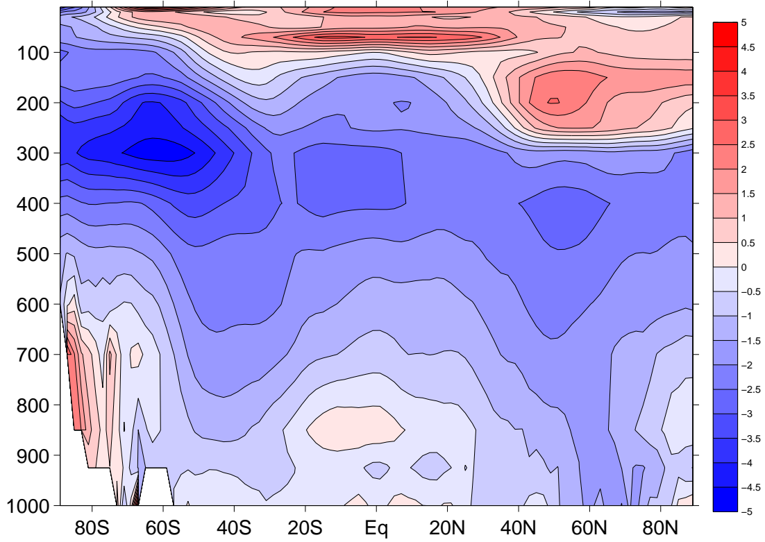
Figure 1. Long-term annual and zonal mean temperature difference between NCEP/NCAR reanalysis climatology and AM2/LM2 (AM2/LM2 minus NCEP). Contour interval is 0.5 K.
